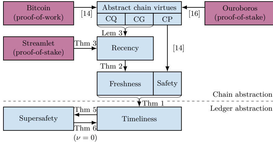
Fig. 1: Paper overview. Bitcoin and Ouroboros attain the abstract chain virtues of Common Prefix, Chain Quality, and Chain Growth (top) [14, 16]. We show that CQ and CG imply the intermediate property of recency (Lemma 3, middle). Recency is also achieved by Streamlet (Theorem 3, middle) and is sufficient to prove freshness (Theorem 2, middle). Freshness, together with safety, is sufficient to prove timeliness (Theorem 1). In safe and live protocols, from timeliness we can achieve supersafety and vice versa (Theorems 5-6, bottom).
